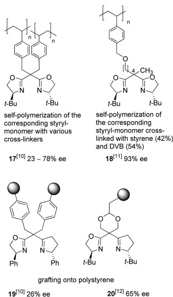
Figure 2. Enantioselectivities of the major trans -diastereomer 21 obtained for the cyclopropanation of styrene ( 12 ) with ethyl diazoacetate with polystyrene-immobilized bis(oxazoline) ligands. [10–12]
