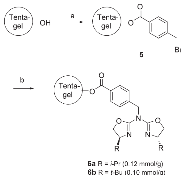
Scheme 1. Synthesis of Tentagel TM -bound azabis(oxazolines). Reagents and conditions: a) 4-(bromomethyl)benzoyl chloride (10 equivs.), pyridine (40 equivs.), CH 2 Cl 2 , room temperature, 48 h, 46%; b) i) 2 (3 equivs.), n -BuLi (3.3. equivs.), THF, –78 °C, 10 min; ii) 5 (1 equiv.), THF, room temperature, 72 h, 85% ( 6a ), 71% ( 6b ).
